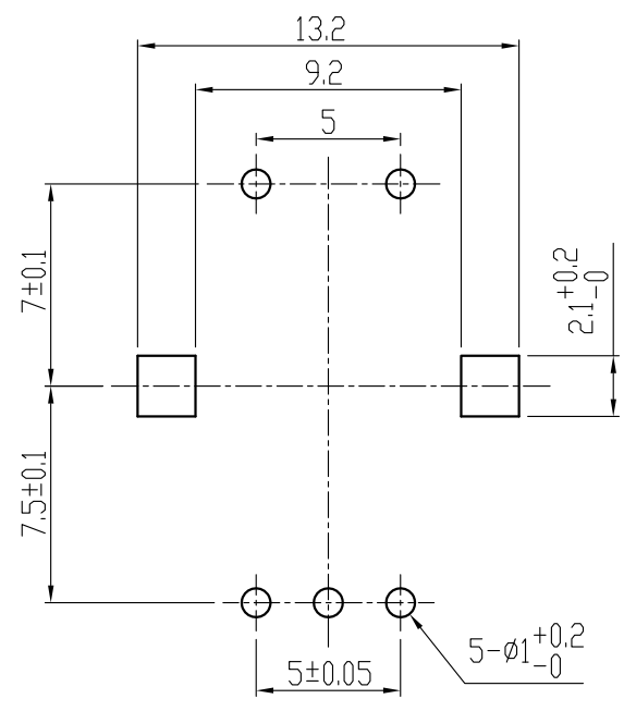
P.C.B.MOUNTING DETAIL
